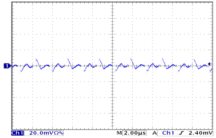
Figure 20: Output voltage ripple at nominal input voltage and rated load current (20mV/div). Load capacitance: 1 \mu F ceramic capacitor and 10 \mu F tantalum capacitor. Bandwidth: 20MHz. See Figure 17.
