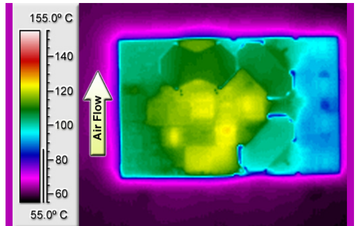
Figure 6: Thermal plot of converter at 6.7 amp load current with 55°C air flowing at the rate of 200 LFM. Air is flowing across the converter sideways from pin 3 to pin 1 (24V input).
