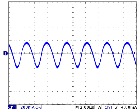
Figure 18: Input Terminal Ripple Current, i_c , at full rated output current and nominal input voltage with 10 \mu H source impedance and 47 \mu F electrolytic capacitor (200mA/div). See Figure 17.
