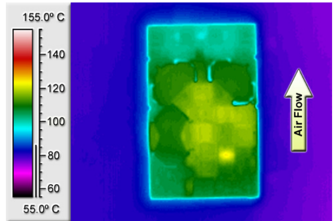
Figure 10: Thermal plot of converter at 5.1 amp load current with 85°C air flowing at the rate of 200 LFM. Air is flowing across the converter from input to output (24V input).
