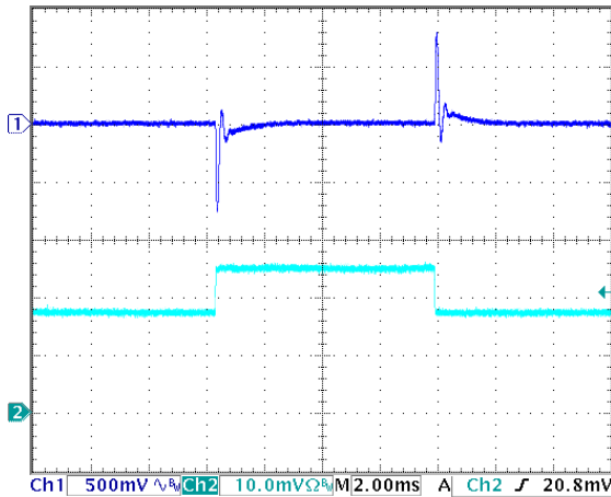
Figure 15: Output voltage response to step-change in load current (50%-75%-50% of Iout(max); dI/dt = 0.1A/\mu s ). Load cap: 10 \mu F , 100 m \Omega ESR tantalum cap and 1 \mu F ceramic cap. Ch 1: Vout (500mV/div), Ch 2: Iout (2A/div).
