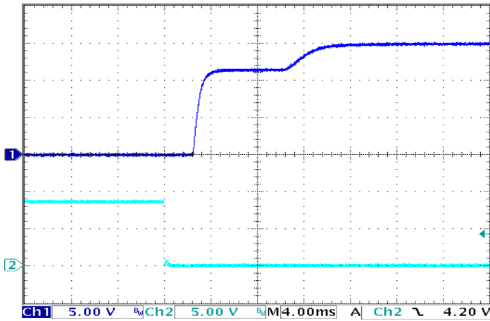
Figure 13: Turn-on transient at full load (resistive load) (4 ms/div). Input voltage pre-applied. Ch 1: Vout (5V/div). Ch 2: ON/OFF input (5V/div).
