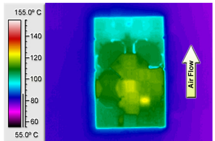
Figure 12: Thermal plot of converter at 4.2 amp load current with 85°C air flowing at the rate of 200 LFM. Air is flowing across the converter from input to output (48V input).
