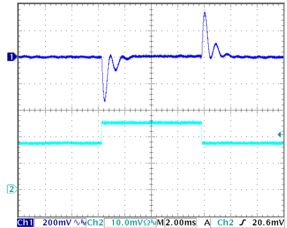
Figure 16: Output voltage response to step-change in load current (50%-75%-50% of Iout(max); dI/dt = 5A/\mu s ). Load cap: 470 \mu F , 30m \Omega ESR tantalum cap and 1 \mu F ceramic cap. Ch 1: Vout (200mV/div), Ch 2: Iout (2A/div).
