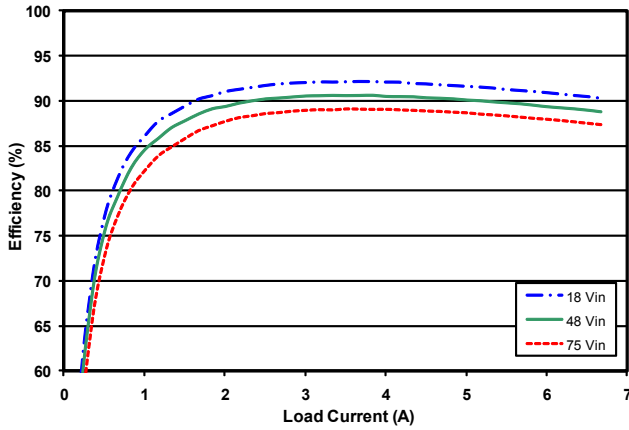
Figure 1: Efficiency at nominal output voltage vs. load current for 18V, 48V and 75V input at 25°C.
