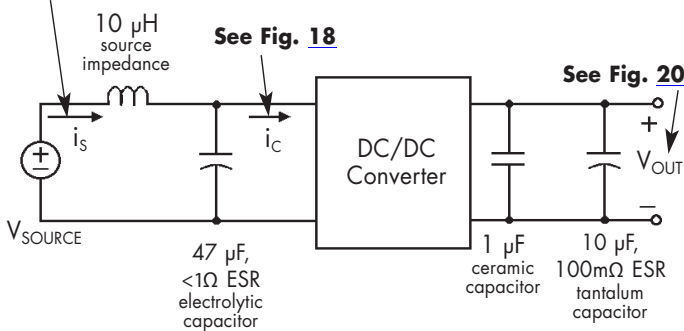
Figure 17: Test set-up diagram showing measurement points for Input Terminal Ripple Current (Fig 18), Input Reflected Ripple Current (Fig 19) and Output Voltage Ripple (Fig 20).
