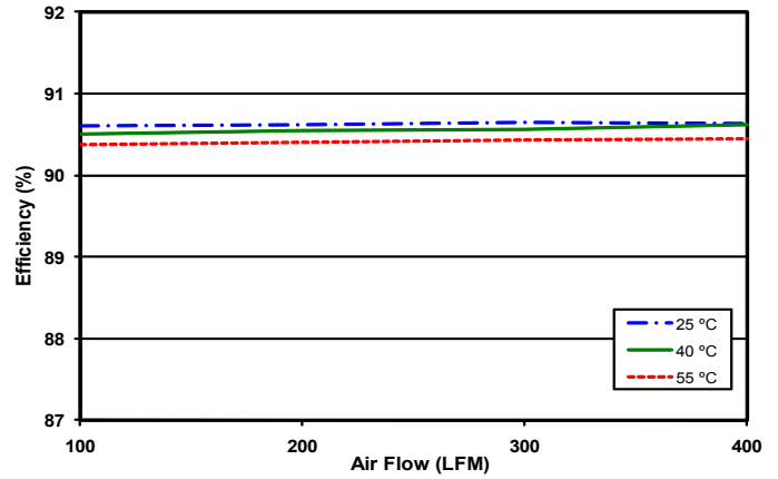
Figure 2: Efficiency at nominal output voltage and 60% rated power vs. airflow rate for ambient air temperatures of 25°C, 40°C, and 55°C (nominal input voltage, 48V input).
