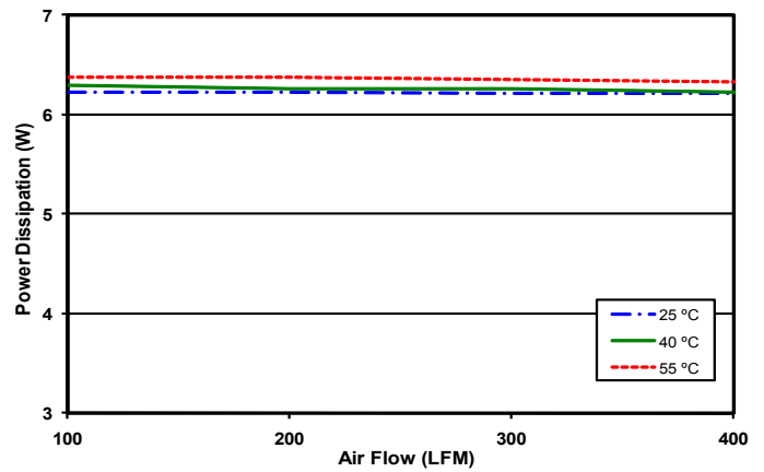
Figure 4: Power dissipation at nominal output voltage and 60% rated power vs. airflow rate for ambient air temperatures of 25°C, 40°C, and 55°C (nominal input voltage, 48V input).
