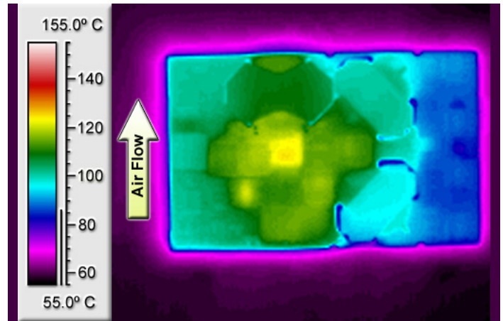
Figure 8: Thermal plot of converter at 6.2 amp load current with 55°C air flowing at the rate of 200 LFM. Air is flowing across the converter sideways from pin 3 to pin 1 (48V input).
